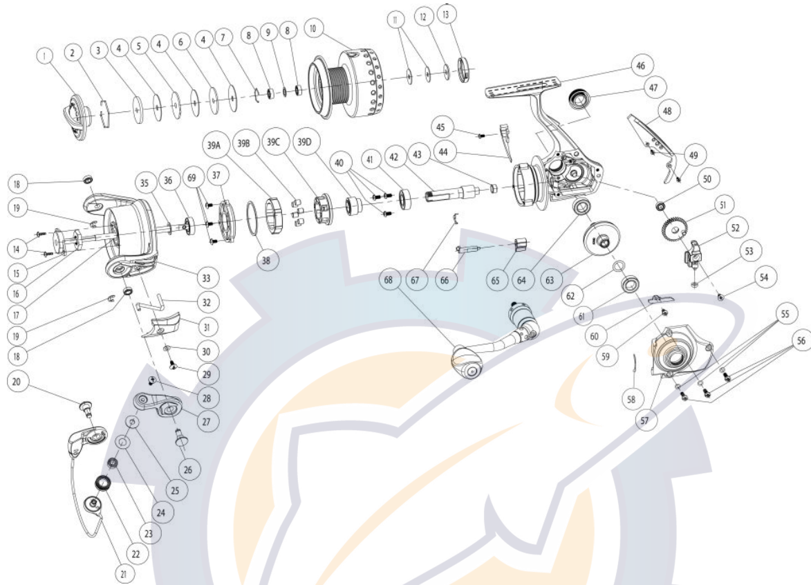
Quantum Energy E40PTIB Spinning Reel Part List
